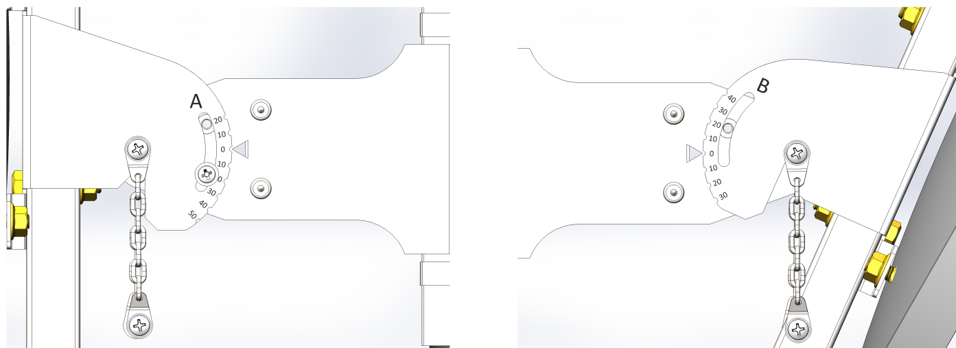
Figure 32 – "A" and "B" scales on the movable part of the bracket
