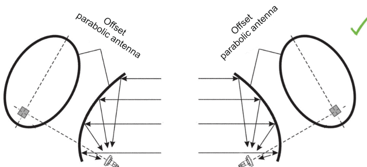
Figure 7 – Correct installation of offset parabolic antennas at the same suspension height
