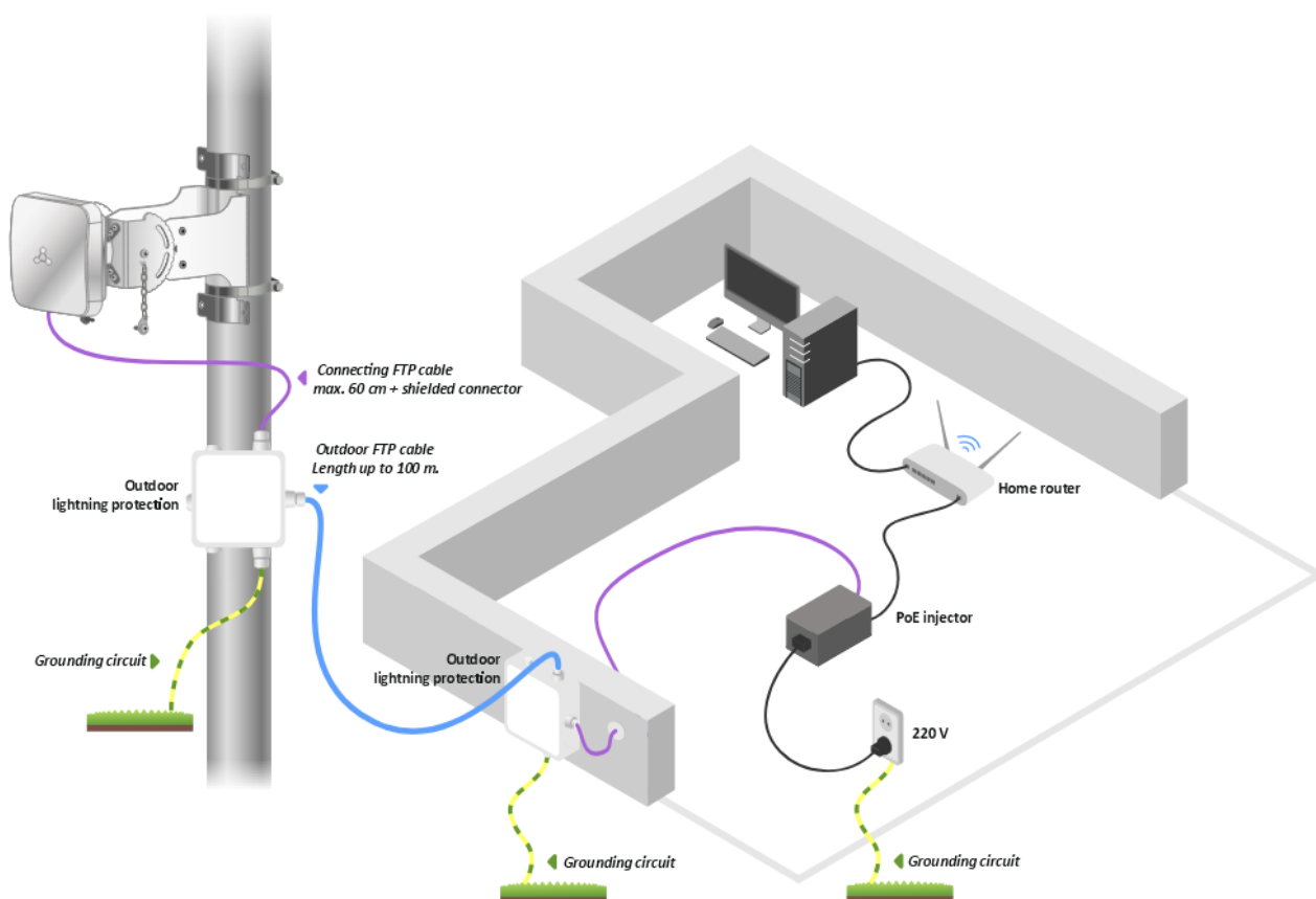
Figure 9 – Device wiring diagram for lightning protection
