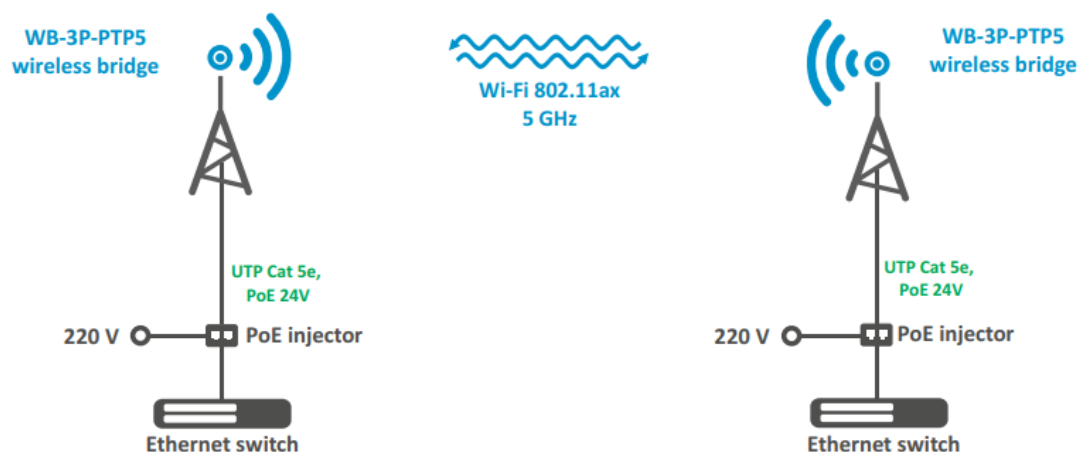
Figure 1 — WB-3P-PTP5 application diagram
