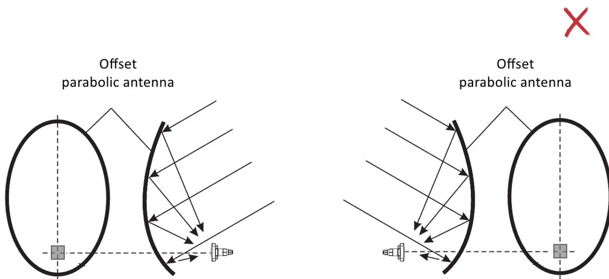
Figure 6 – Incorrect installation of offset parabolic antennas
